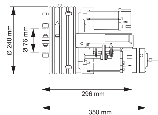
Dimensiones (mm) TIGER T210 / T420
